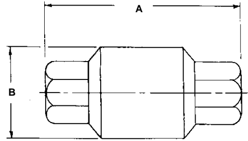
3/8" - 3/4" BODY
