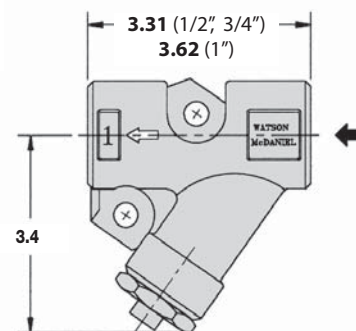
UC450SL (Strainer)
