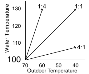
Reset Ratio Curves
