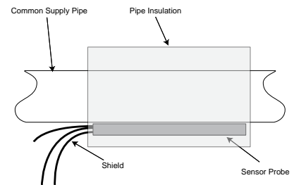
Strap-On Heating System Sensor
